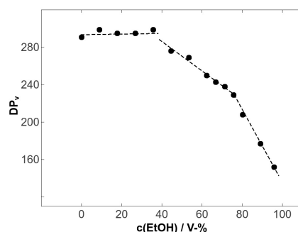
Figure 1: DPv of HCS-Domsjö pulp with various ethanol concentrations in HyCellSolv-treatment (dashed lines are given to guide the eye, indicating the three possible regions of depolymerisation kinetics)
