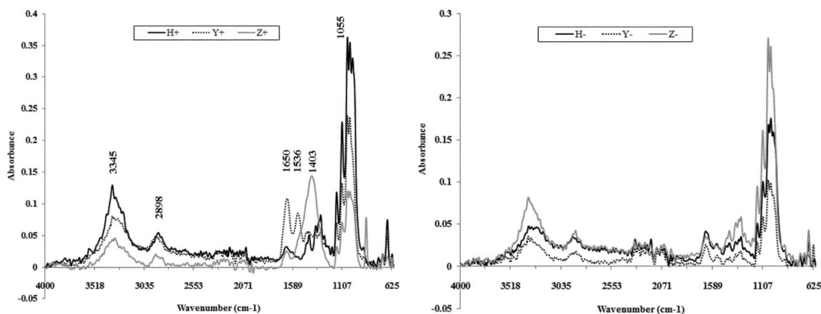
Figure 4: FTIR spectra of BC
