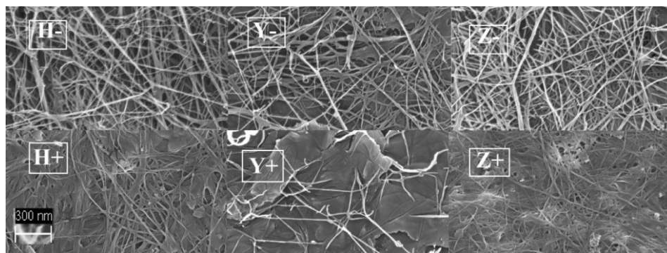
Figure2: FE-SEM micrographs of BC produced under agitation from different media (H, Y and Z) in the presence (+) or absence (-) of ethanol
