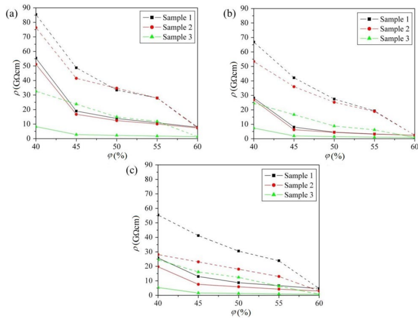
Figure 6: Hysteresis of knitted fabrics' volume resistivity ( \rho ) as a function of humidity ( \phi ): (a) before pilling; (b) after pilling with the investigated knitted fabric (7000 rubs); (c) after pilling with the wool woven fabric (7000 rubs); (--- sorption curve; — desorption curve)
