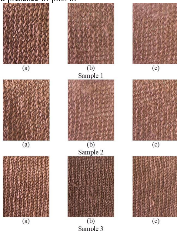
Figure 4: Surface appearance of plain knitted fabrics at 5\times magnification: (a) before pilling; (b) after pilling with the investigated knitted fabric (7000 rubs); (c) after pilling with the wool woven fabric (7000 rubs)
