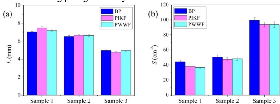
Figure 2: Structural characteristics of knitted fabrics before and after pilling: (a) loop length ( L ), (b) stitch density ( S ); (BP – before pilling; PIKF – pilling caused by the investigated knitted fabric; PWVF – pilling caused by the wool woven fabric)
