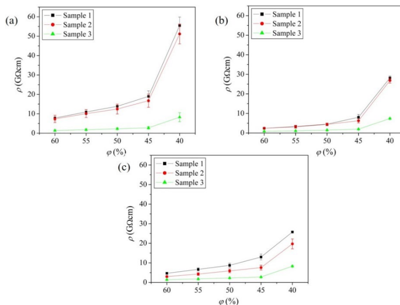
Figure 5: Influence of humidity ( \varphi ) on knitted fabrics' volume resistivity ( \rho ): (a) before pilling; (b) after pilling with the investigated knitted fabric (7000 rubs); (c) after pilling with the wool woven fabric (7000 rubs)
