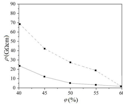
Figure 1: Hysteresis of the textile materials volume resistivity ( \rho ) as a function of humidity ( \varphi ); (- - sorption curve; — desorption curve)
