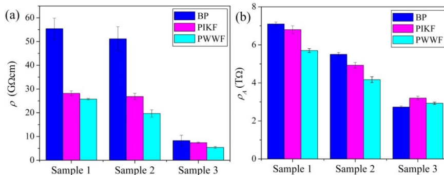
Figure 3: Electrical resistivities of knitted fabrics before and after pilling: (a) volume resistivity ( \rho ), (b) surface resistivity ( \rho_A ); BP – before pilling; PIKF – pilling caused by the investigated knitted fabric; PWWF – pilling caused by the wool woven fabric)
