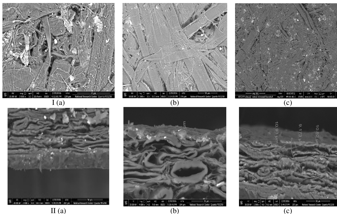
Figure 5: SEM images of surfaces (I) and edges (II) of paper sheets (a) uncoated, (b) coated with 30 CNF, and (c) coated with 30 CNF/shellac
