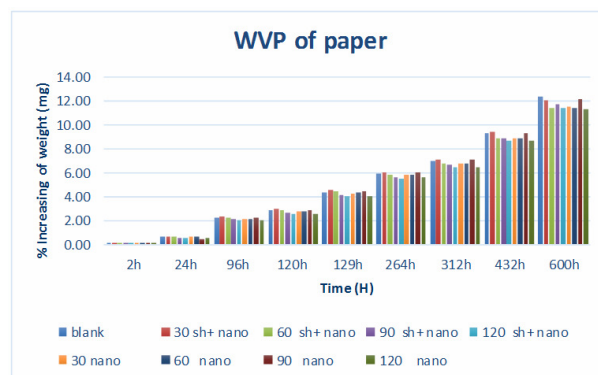
Figure 4: Water vapour permeability of papers coated with CNF and CNF/shellac films of various thicknesses
