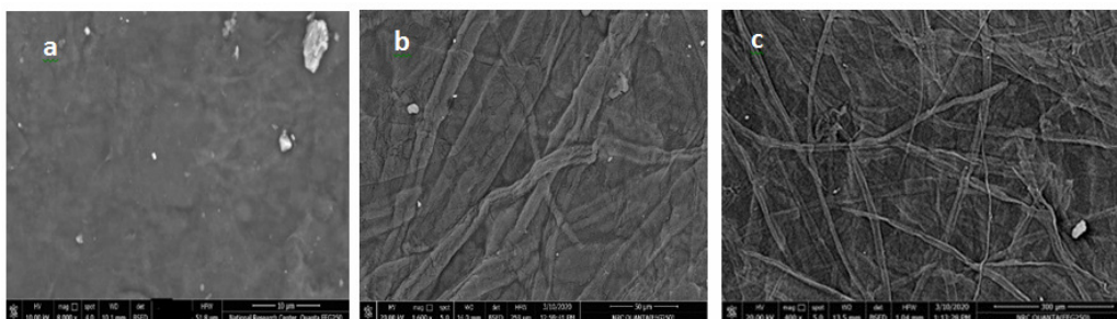
Figure 2: Scanning electron micrographs (SEM) of CNF and shellac nanocomposite films; (a) CNF, (b) 5% shellac and 95% CNF, (c) 40% shellac and 60% CNF
