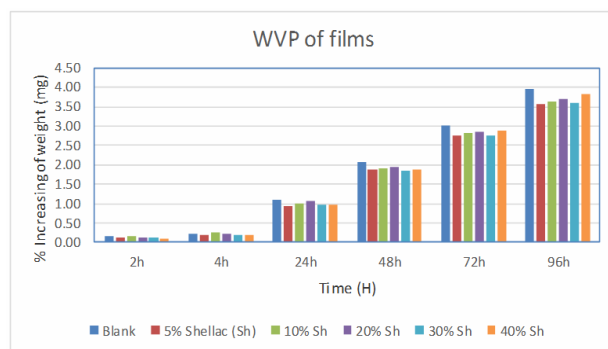
Figure 3: Water vapor permeability of different CNF and CNF/shellac films
