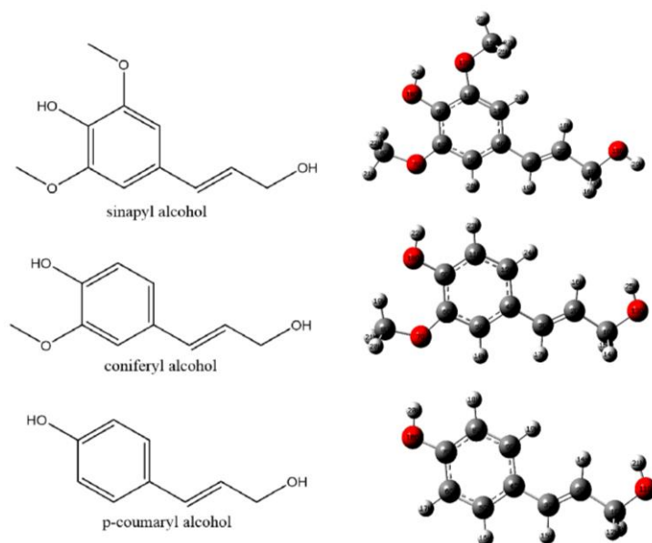
Figure 1: Optimized molecular structure of monolignols
