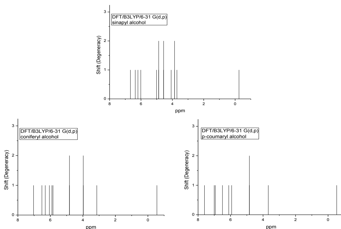
Figure 3: Calculated ^1\text{H} -NMR of monolignols
