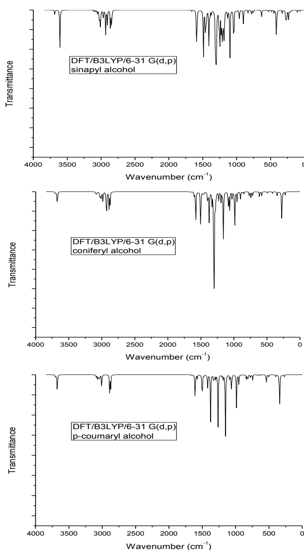
Figure 2: Calculated vibrational frequencies of monolignols
