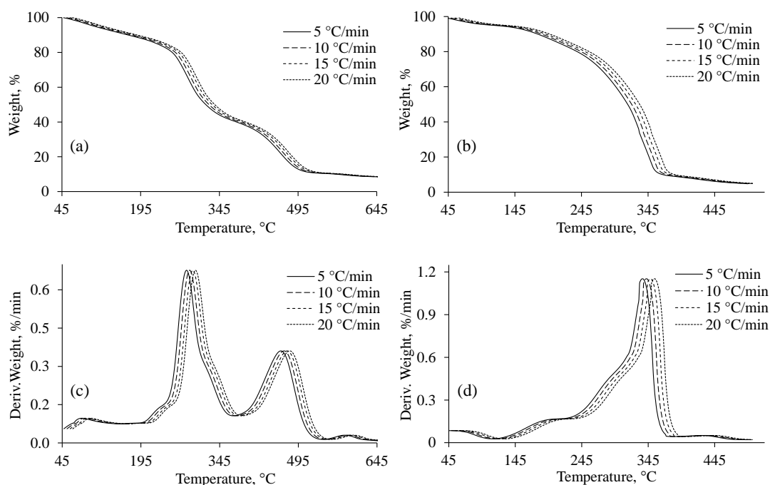
Figure 4: Overlaid TG and DTG curves of LSH (a, c) and ALSH 3 (b, d), respectively, recorded at multiple heating rates
