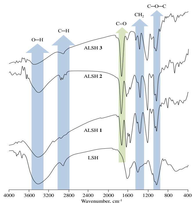
Figure 1: FTIR spectra of LSH, ALSH 1, ALSH 2 and ALSH 3
