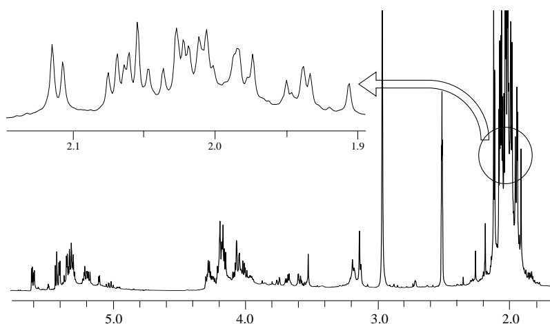
Figure 3: ^1\text{H} NMR spectrum of ALSH 3 (DS 2.91), (600 MHz, ppm, \text{DMSO-}d_6 , 40 ^\circ\text{C} )
