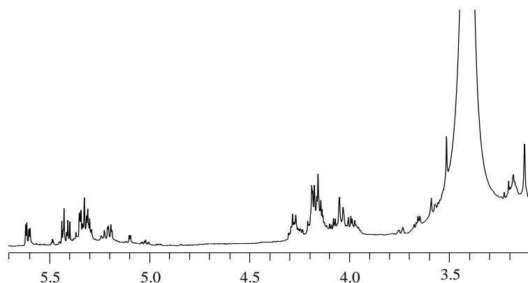
Figure 2: ^1\text{H} NMR spectrum of LSH (600 MHz, ppm, \text{DMSO-}d_6 , 40 ^\circ\text{C} )
