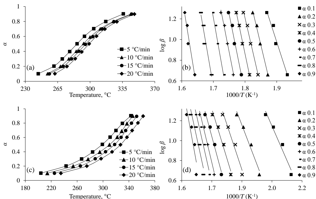
Figure 5: \alpha vs. T plots of thermal degradation of LSH (a) and ALSH 3 (c) at multiple heating rates and Flynn-Wall-Ozawa (FWO) plots between \log \beta and 1000/T ( K^{-1} ) for calculation of E_a of degradation steps at several degrees of conversion for LSH (b) and ALSH 3 (d)
