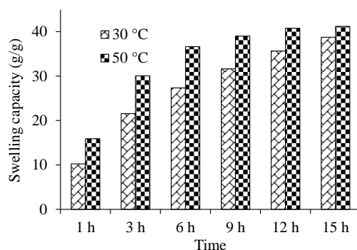
Figure 6: Swelling capacity of LSH at 30 °C and 50 °C
