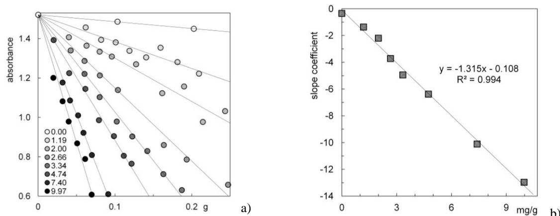
Figure 2: (a) Absorbance of the dye solution at equilibrium vs. mass of cotton sample with indicated PHMB content (mg/g) and (b) the corresponding plot slopes vs. PHMB content
