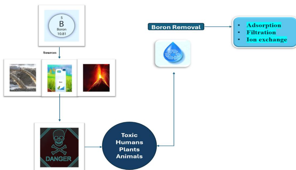
Figure 1: Sources, toxicity and removal methods of boron from water
