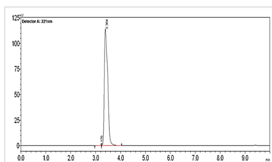
Figure 6: HPLC chromatogram of empagliflozin (3.3 min) in plasma
