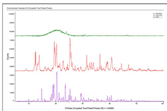
Figure 9: XRD overlay of transferosomal buccal film (TFS)
