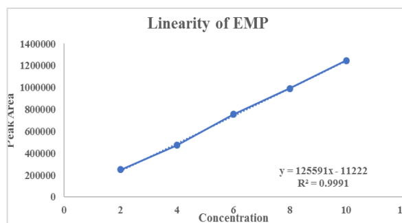
Figure 7: Standard calibration curve of EMP in plasma
