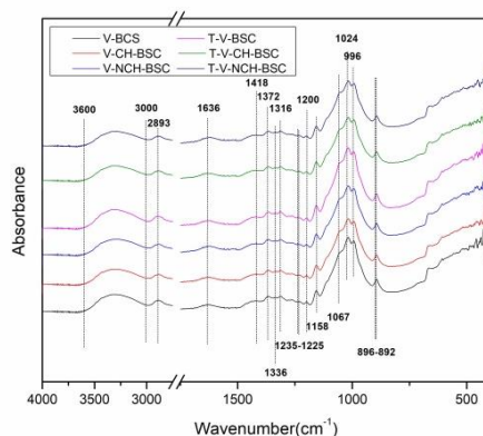
Figure 3: FTIR spectra of fabrics after functionalization with BSC, in the wavenumber range of 400\text{--}4000\text{ cm}^{-1}
