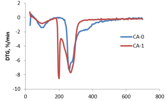
Figure 7: Results of differential thermogravimetric analysis (DTG curves) of samples
