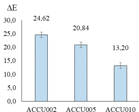
Figure 8: Color difference between cotton samples dyed at 0.2, 0.5 and 1.0% owf of \text{CuSO}_4 \cdot 5\text{H}_2\text{O} at a DR of 80/20, 60 °C, and 60 min (no pH adjustment), after a washing cycle
