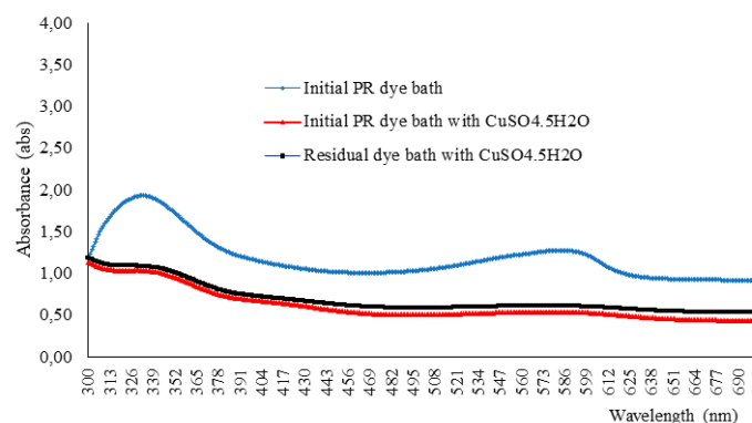
Figure 7: UV-Vis spectra of residual PR dye bath after dyeing cotton with 0.5% owf of \text{CuSO}_4 \cdot 5\text{H}_2\text{O}
