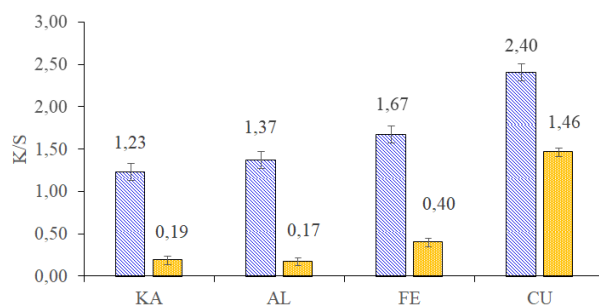
Figure 6: K/S values of cotton fabrics dyed with PR extract and mordanted with \text{KAl}(\text{SO}_4)_2 \cdot 12\text{H}_2\text{O} (KA), \text{Al}_2(\text{SO}_4)_3 \cdot 18\text{H}_2\text{O} (AL), \text{FeSO}_4 \cdot 7\text{H}_2\text{O} (FE), and \text{CuSO}_4 \cdot 5\text{H}_2\text{O} (CU), before and after washing
