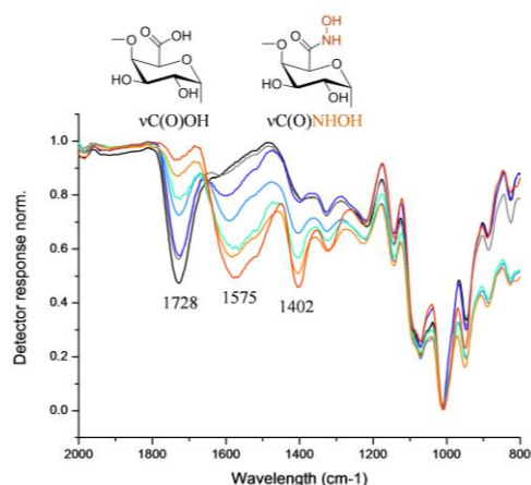
Figure 1: FTIR spectra (ATR) of polygalacturonic hydroxamic acids with increasing hydroxamic acid content
