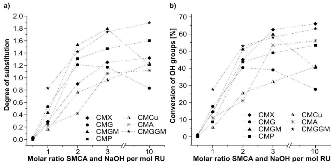
Figure 2: Degrees of substitution of different carboxymethyl (CM) polysaccharides (a) and the conversion of available hydroxyl groups per anhydrosugar unit (b) obtained by the conversion of different polysaccharides with sodium monochloroacetate (SMCA) and aqueous NaOH using varying molar ratios (X: xylan, G: \alpha -1,3-glucan, GM: glucomannan, P: pullulan, Cu: curdian, A: agarose, GGM: galactoglucomannan)
