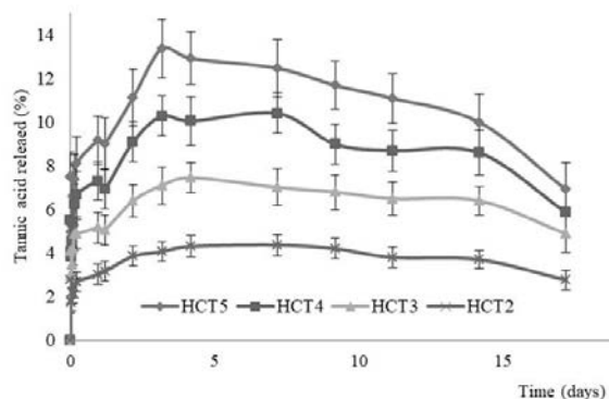
Figure 9: Tannic acid release from HC-TA films
