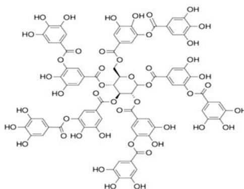
Figure 1: Tannic acid chemical structure
