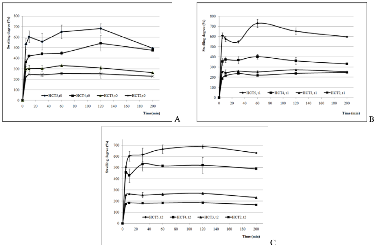
Figure 6: Variation in time of the swelling degree in double distilled water of HC/TA hydrogels of different HC-TA ratio and different crosslinking time intervals, (A) t_0 , (B) t_1 and (C) t_2
