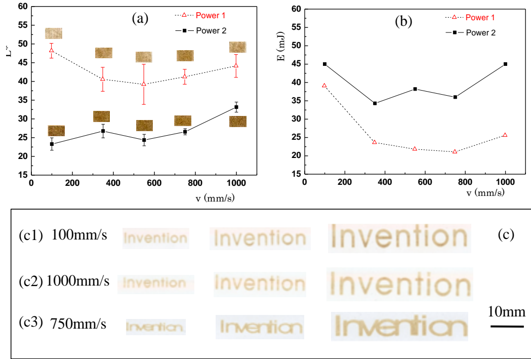
Figure 4: Relationship between the degree of yellow discoloration and LIEP parameters: (a) brightness values L^* of the color blocks; (b) laser energy; (c) samples printed with different LIEP parameters for power 1 (c1, c2) and power 2 (c3)
