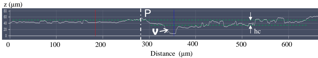
Figure 5: Unevenness of the printing paper surface for a velocity of 350 mm/s and a power of 3 W (magnification: 2000x)
