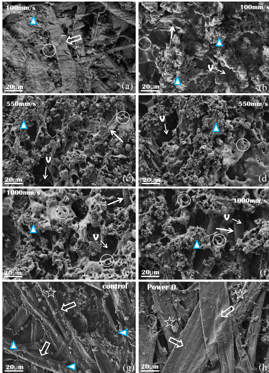
Figure 2: Typical carbonized microstructure and control sample: (a-c) power 1 and (d-f) power 2
