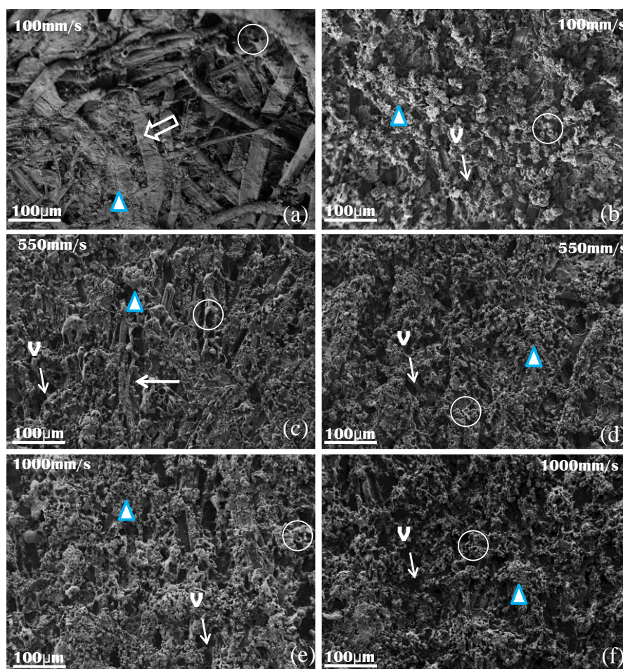
Figure 1: Low-magnification SEM images of the carbonized microstructure of paper after LIEP: (a-c) power 1 and (d-f) power 2
