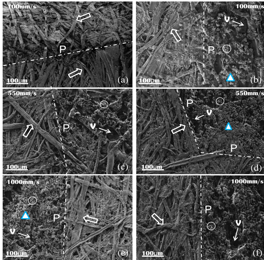
Figure 3: Carbonized microstructures of the boundary of LIEP: (a-c) power 1 and (d-f) power 2
