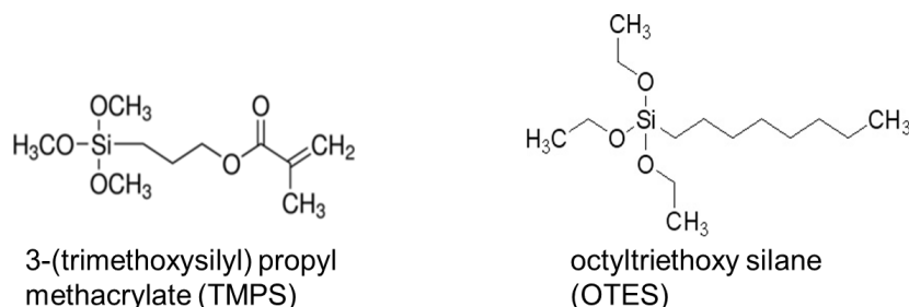
Figure 1: Chemical structure of the organotrialkoxysilane coupling agents used in the study to chemically modify abaca fibers
