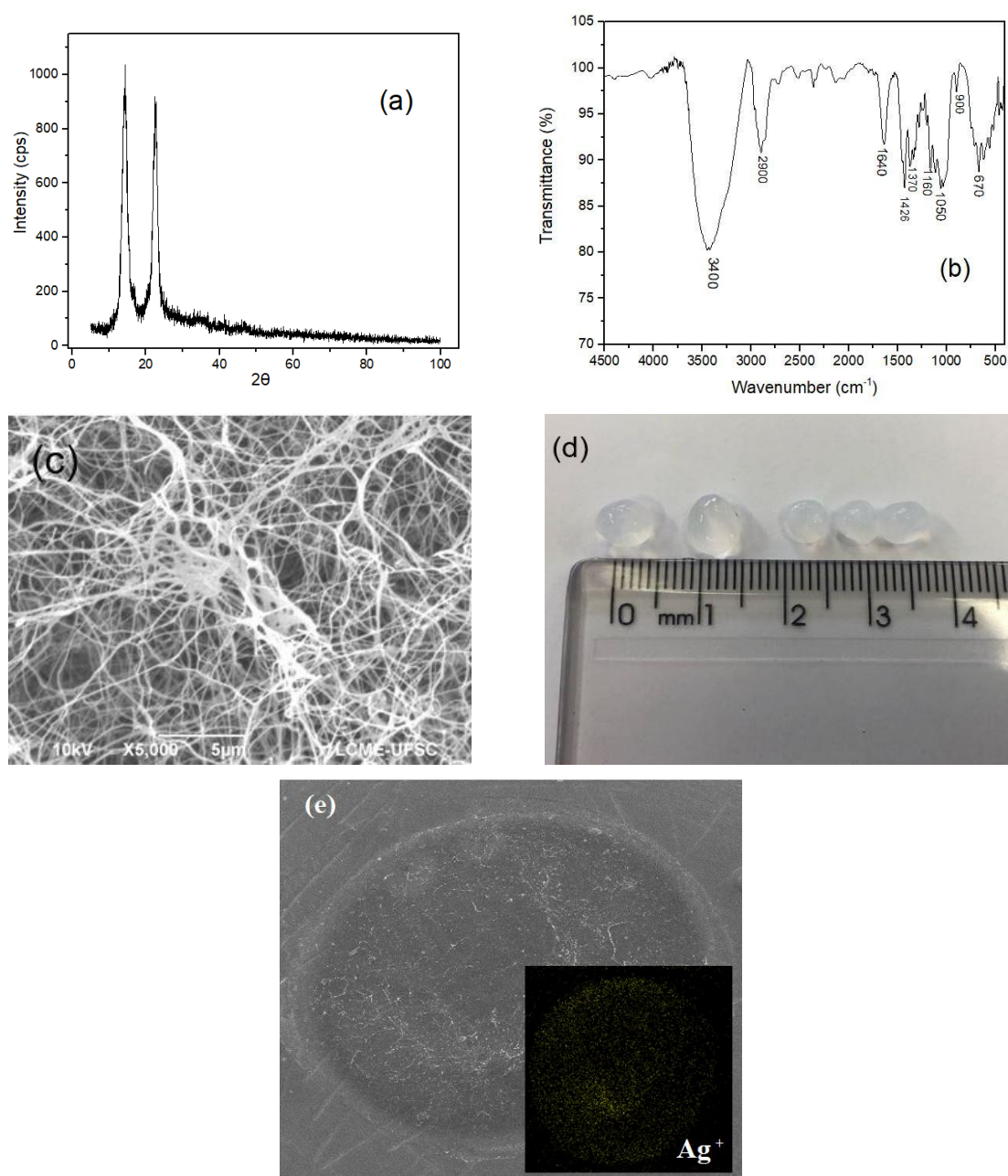
Figure 1: Characterization of bacterial nanocellulose spheres; (a) XRD, (b) FTIR, (c) MEV, and (d) photograph of BNCs; (e) elemental mapping before and after (inset) adsorption of Ag +
